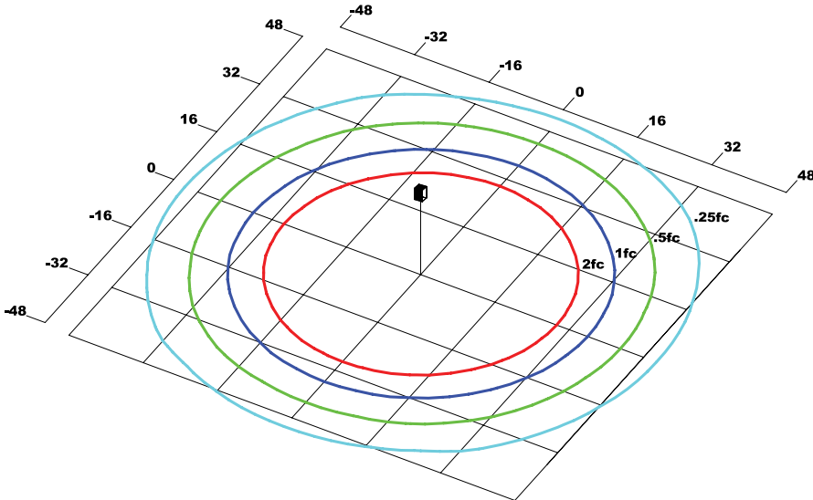
EESCP20QF1X186U 5KC Type V Grid in MH MH=16 Feet
