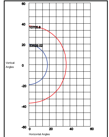
EES-SP52Q55536U5K 38°H x 39°V Beam, NEMA 5H x 5V
